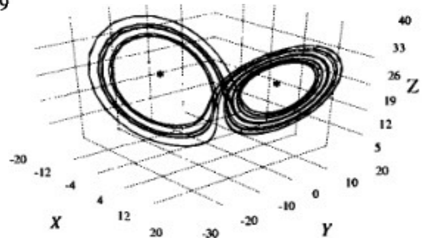
Fig. 1.19. Solutions to the Lorenz equations for r = 25 . The initial point was X = 0, Y = -5, Z = 15 . In the state space diagram in the lower right panel, the two off-origin fixed points at Z = 24, X = 8 and Y = 8 are indicated by asterisks.
