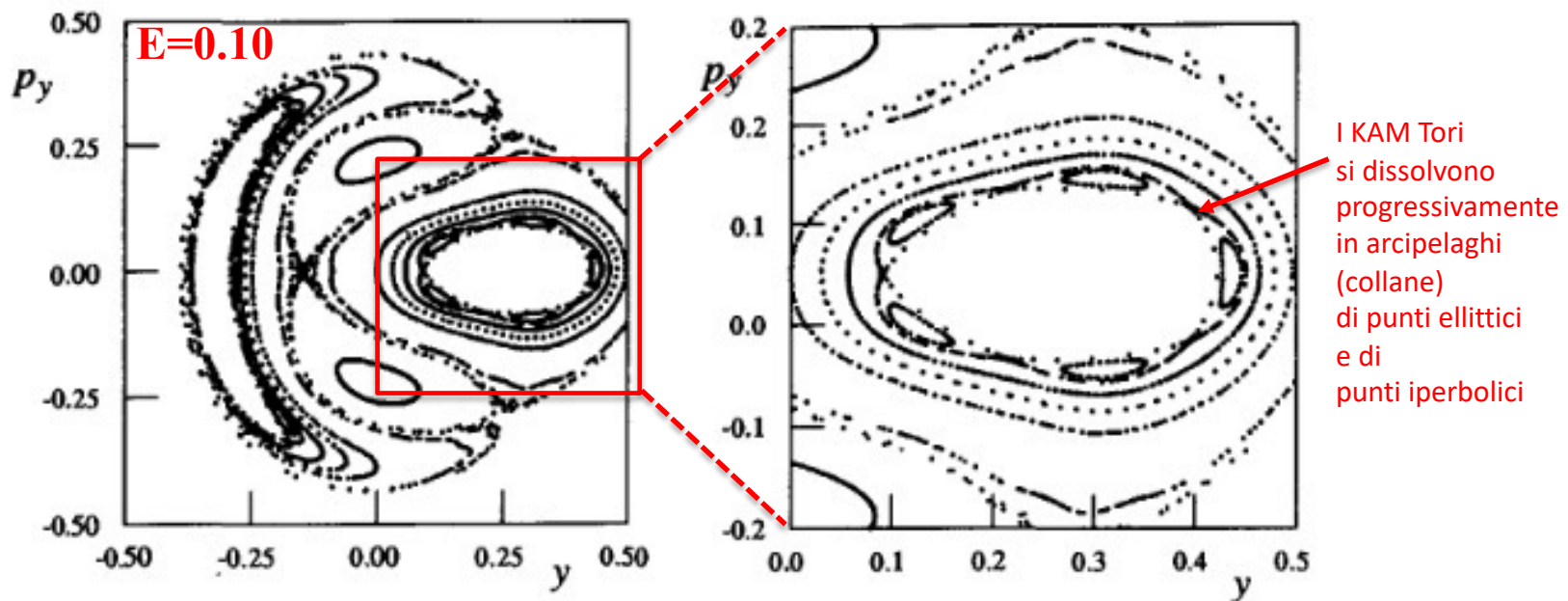
Fig. 8.13. On the left is the Poincaré section for the Hénon–Heiles model with E = 0.10 . On the right is a magnified view of one of the archipelago island chains of elliptic and hyperbolic points that form from a KAM torus. Surrounding this chain are other surviving KAM tori.
