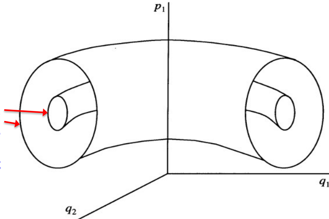
Fig. 8.5. For an integrable two-degree-of-freedom system, the trajectories are confined to the surfaces of a set of nested tori. Each surface corresponds to a different set of values of the two constants of the motion. If the system becomes nonintegrable, the trajectories can move off the tori.
