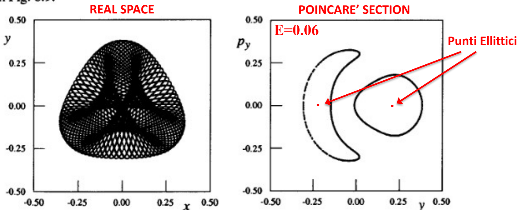
Fig. 8.9. On the left is the xy (real space) trajectory of a particle moving in the Hénon-Heiles potential with E = 0.06 . The orbit started with x = 0 , y = -0.1475 , p_x = 0.3101 , and p_y = 0 . On the right is the corresponding p_y - y Poincaré section with x = 0 . The “ellipses” are formed by the intersection of the surface of a three-dimensional torus with the Poincaré plane.
