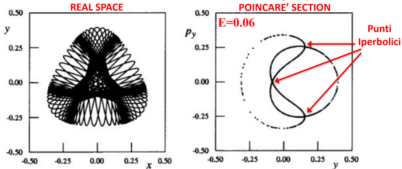
Fig. 8.10. On the left is another orbit of the Hénon–Heiles potential for E = 0.06 , but with initial conditions different from those in Fig. 8.9. On the right is the corresponding y p_y Poincaré section.
