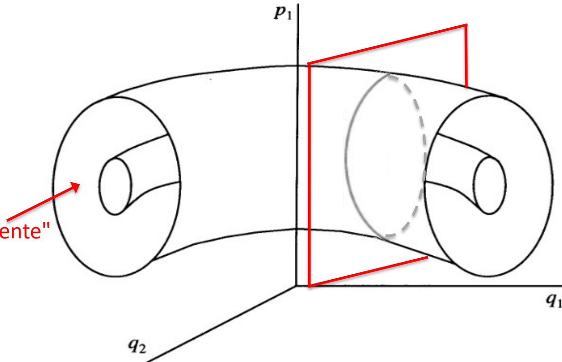
Fig. 8.5. For an integrable two-degree-of-freedom system, the trajectories are confined to the surfaces of a set of nested tori. Each surface corresponds to a different set of values of the two constants of the motion. If the system becomes nonintegrable, the trajectories can move off the tori.
