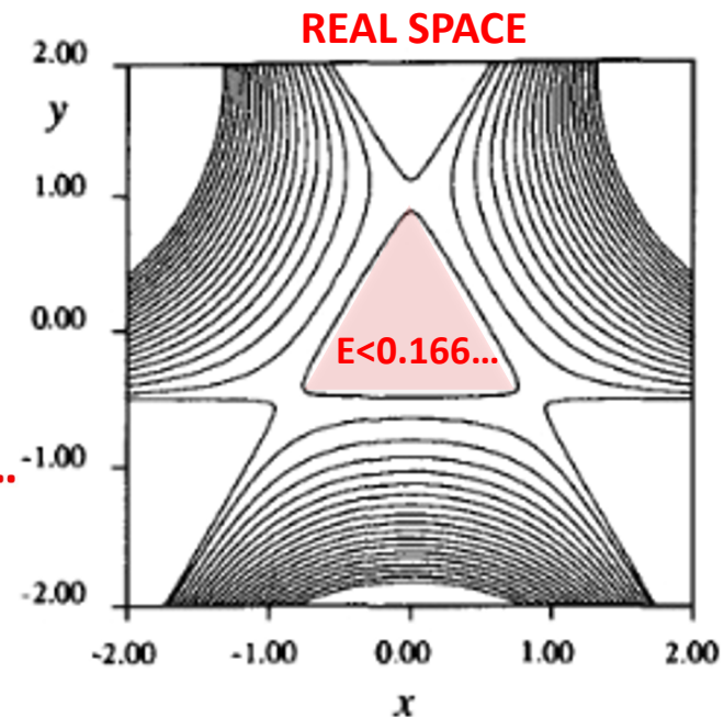
Fig. 8.8. On the left is a three-dimensional plot of the potential energy function for the Hénon-Heiles model. On the right is a contour plot of the same function. We will be concerned with a particle moving in the slight depression near the origin. If the particle's energy is less than 1/6 , the particle will be trapped in the triangular region near the origin. For higher energies the particle can escape the local minimum of the potential energy.
