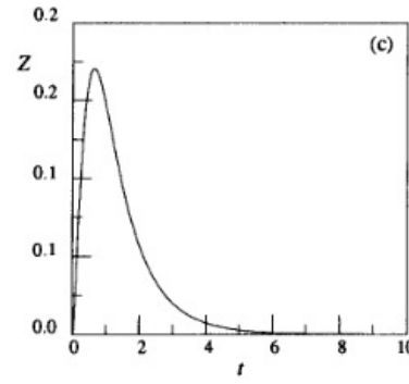
Fig. 1.17. In (a), (b), and (c), X , Y , and Z are plotted as functions of time for the Lorenz model with r = 0.5 , p = 10 , and b = 8/3 . In (d), the trajectory is shown as a projection onto the ZX plane of state space. In all cases the trajectory started at the initial point X = 0 , Y = 1 , Z = 0 .
