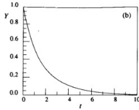
Fig. 1.17. In (a), (b), and (c), X , Y , and Z are plotted as functions of time for the Lorenz model with r = 0.5 , p = 10 , and b = 8/3 . In (d), the trajectory is shown as a projection onto the ZX plane of state space. In all cases the trajectory started at the initial point X = 0 , Y = 1 , Z = 0 .
