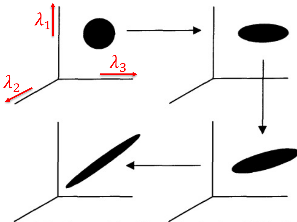
Fig. 4.19. A schematic representation of the evolution of a sphere of initial points in state space. The sphere starts in the upper-left-hand side. Time increases as we go clockwise around the figure. For a dissipative system, the volume associated with the set of initial points must go to 0. A chaotic system will exhibit exponential stretching of the sphere in at least one direction.
