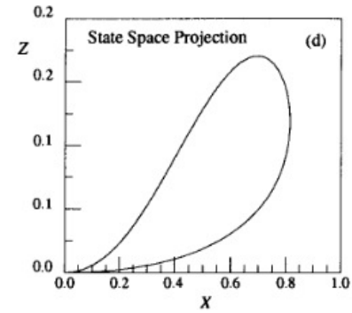
Fig. 1.17. In (a), (b), and (c), X , Y , and Z are plotted as functions of time for the Lorenz model with r = 0.5 , p = 10 , and b = 8/3 . In (d), the trajectory is shown as a projection onto the ZX plane of state space. In all cases the trajectory started at the initial point X = 0 , Y = 1 , Z = 0 .
