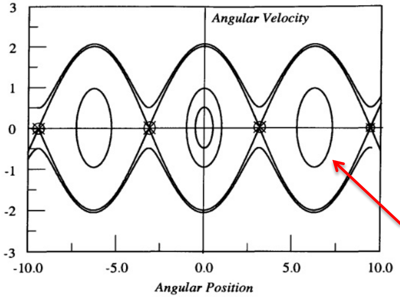
2dim Phase space
