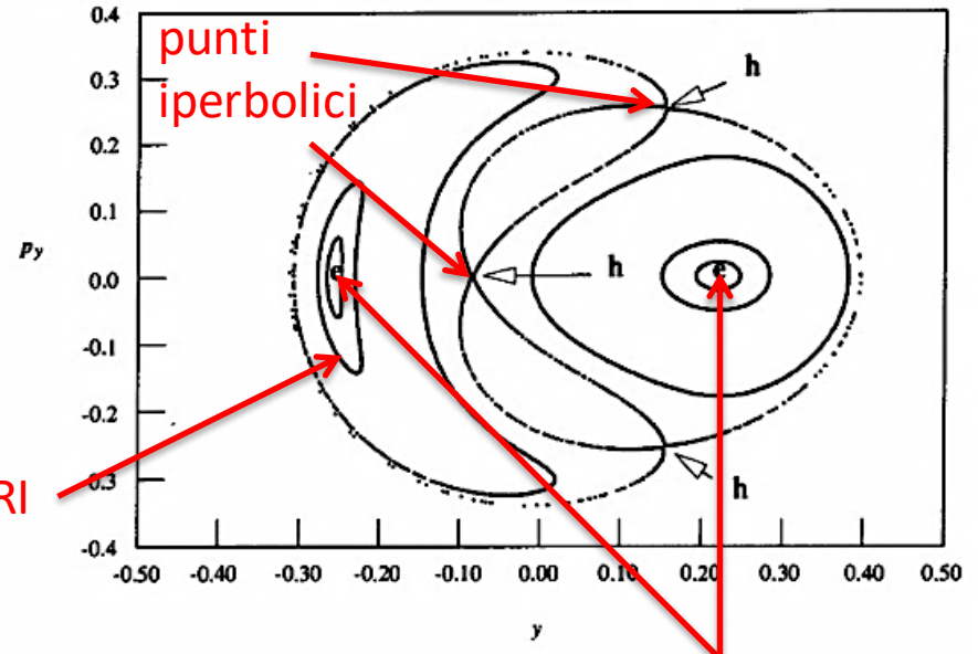
2dim Poincarè section
