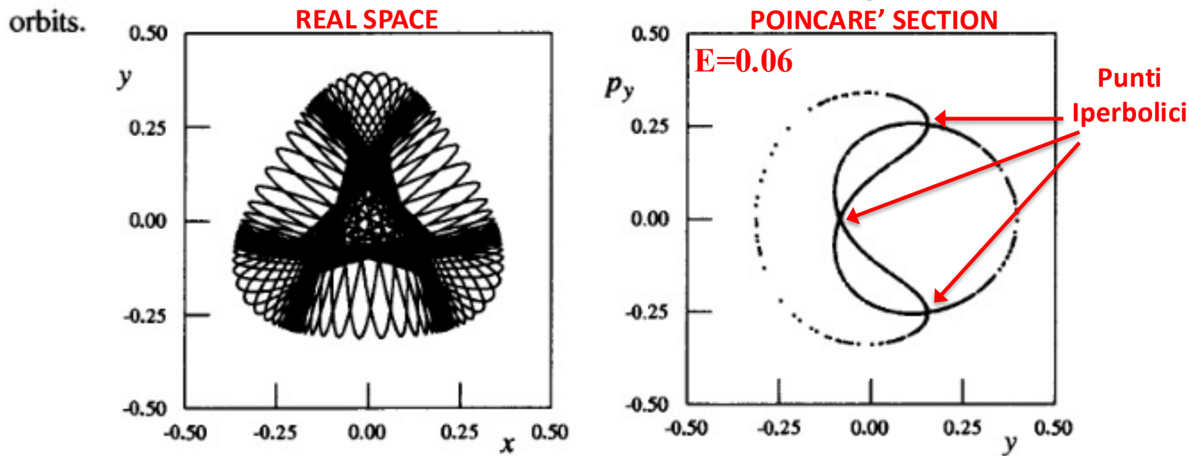
Fig. 8.10. On the left is another orbit of the Hénon–Heiles potential for E = 0.06 , but with initial conditions different from those in Fig. 8.9. On the right is the corresponding y p_y Poincaré section.
